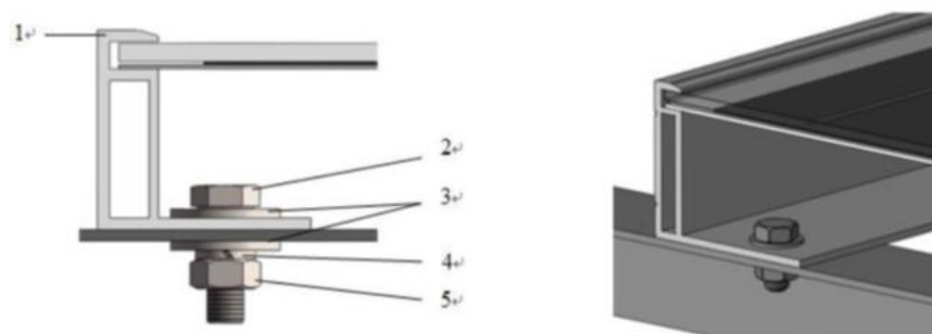
Fig.1 Backsheet-Glass module
